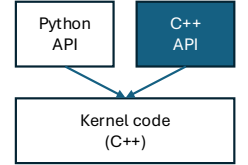
Fig. 1: Layered organization of a Deep Learning Library.
