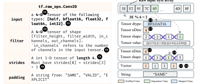
Fig. 7: Illustration of LLM transformation patterns.
